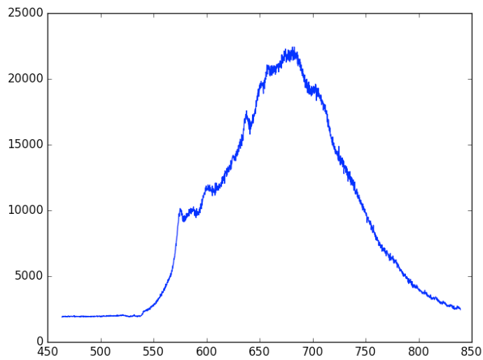
Spectra of NV°/NV- centers with characteristic ZPL lines at 575 and 637nm, respectively.
